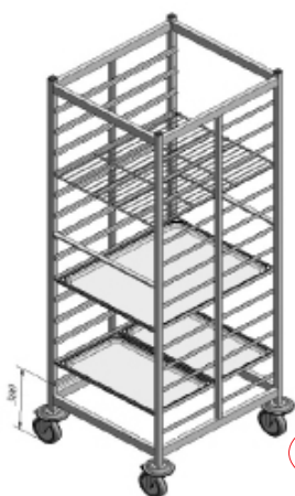
Transportna kolica inox za 14xGN-2/1 ili 28xGN-1/1 GN container trolley for 14xGN-2/1 or 28xGN-1/1, s/s
