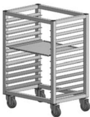
Kolica inox za pekarske tave 434x333 mm Container trolley, s/s, 434x333 mm
